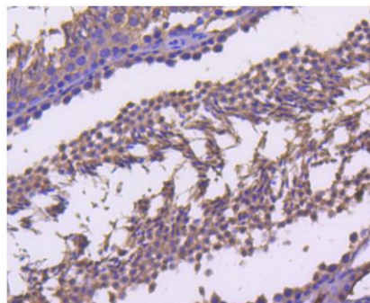
Fig. 3. Immunohistochemical analysis of paraffin-embedded mouse testistissue using anti-Cyclin B2 antibody. Counter stained with hematoxylin.
