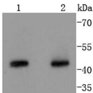
Fig. 1. Western blot analysis of Cyclin B2 on different lysates using anti-Cyclin B2 antibody at 1/1,000 dilution. Positive control: Lane 1: HeLa; Lane 2: K562
