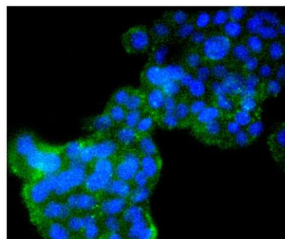
Fig. 2. ICC staining Cyclin B2 in PC-12 cells (green). The nuclear counter stain is DAPI(blue). Cells were fixed in paraformaldehyde, permeabilised with 0.25% Triton X-100/PBS.
